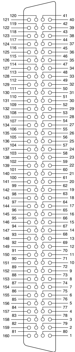
Figure 2. NI 2530B Connector Pinout
